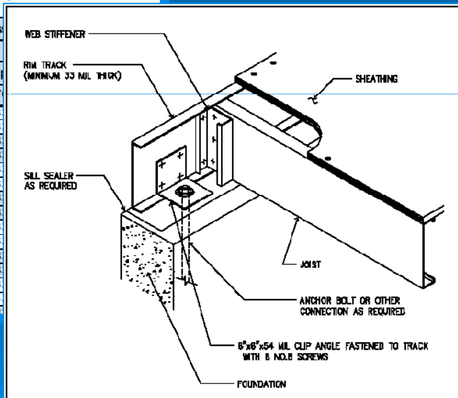
Figure D2-3 Floor to Foundation Connection
